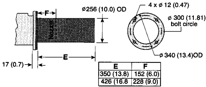
Inverted left hand piping
