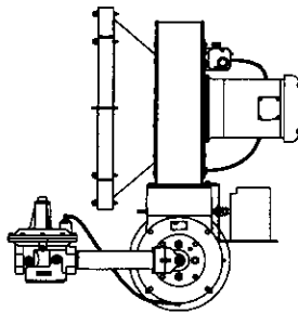
Upright left hand piping
